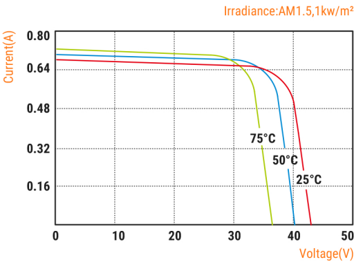
I-V Curves (STC)
